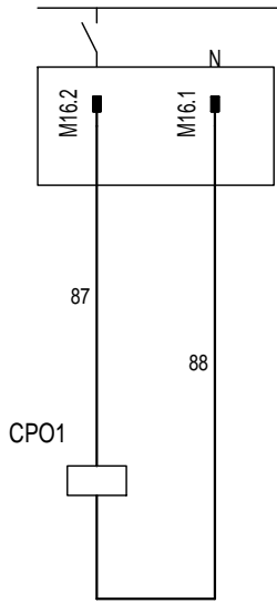
COMANDO POMPA 1 PUMP CONTROL 1
